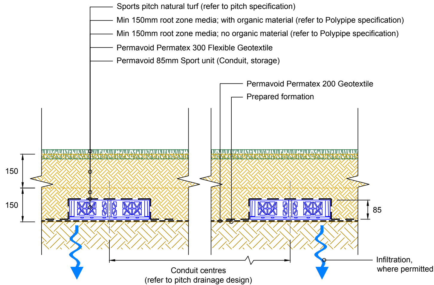
TYPICAL SECTION Scale 1:10
