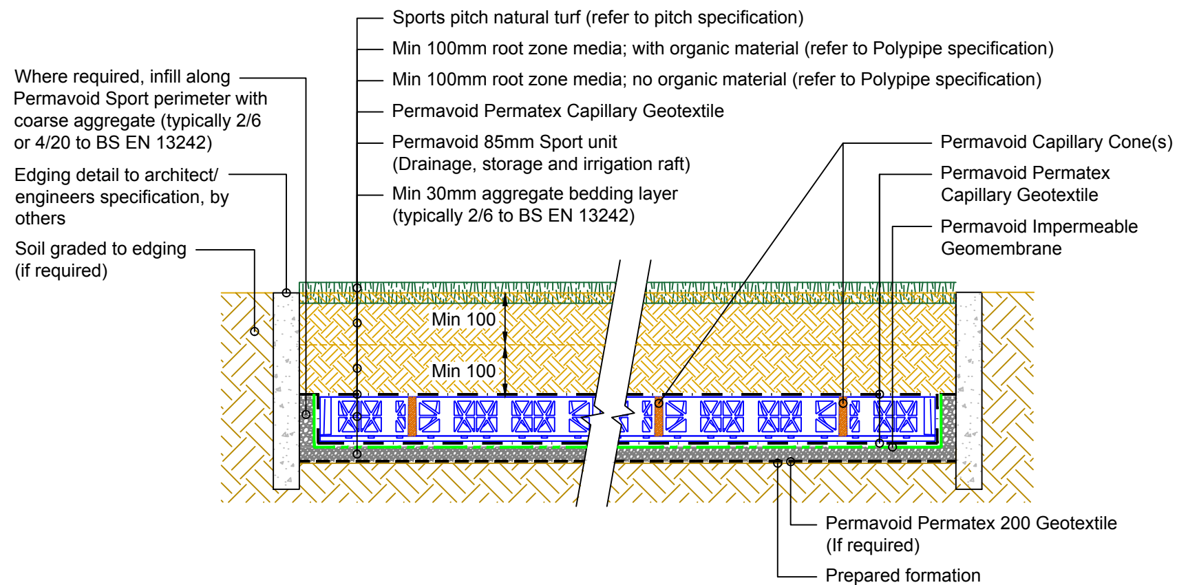
TYPICAL SECTION Scale 1:10
