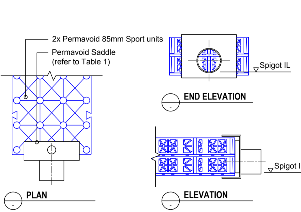
PERMAVOID 85mm SPORT CONDUIT SADDLE CONNECTION Scale 1:10
