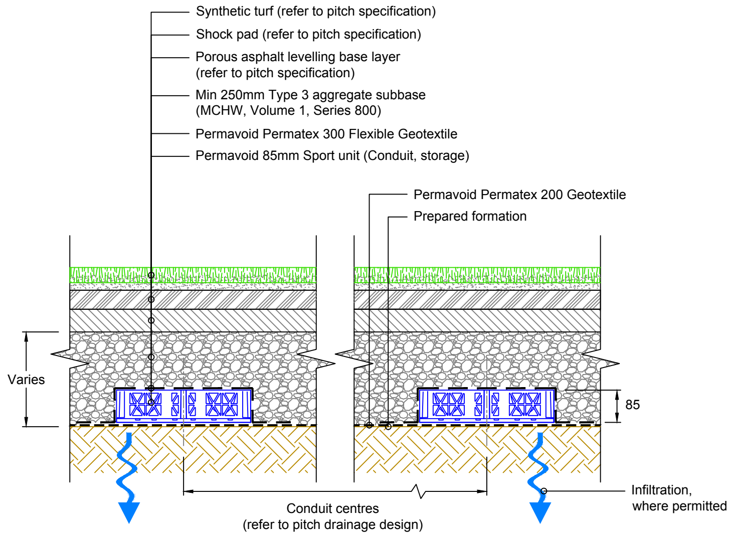
TYPICAL SECTION Scale 1:10
