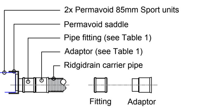
PERMAVOID 85mm SPORT UNIT SADDLE CONNECTION BS EN 1401-1 PIPE Scale 1:20
