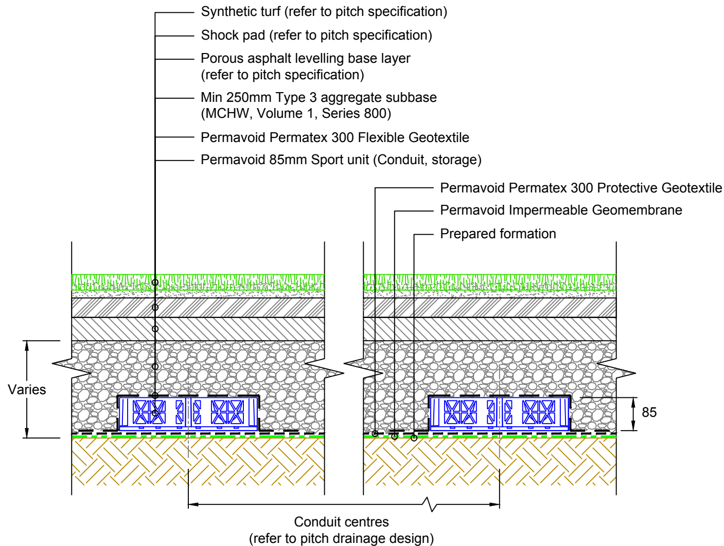
TYPICAL SECTION Scale 1:10
