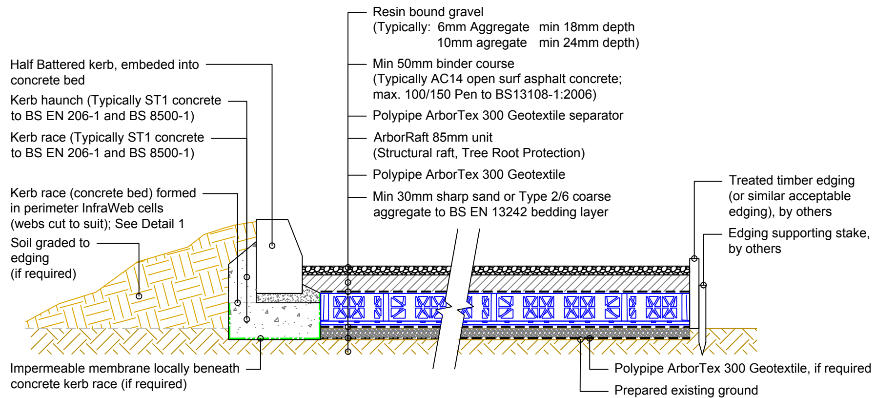
TYPICAL SECTION Scale 1:10
