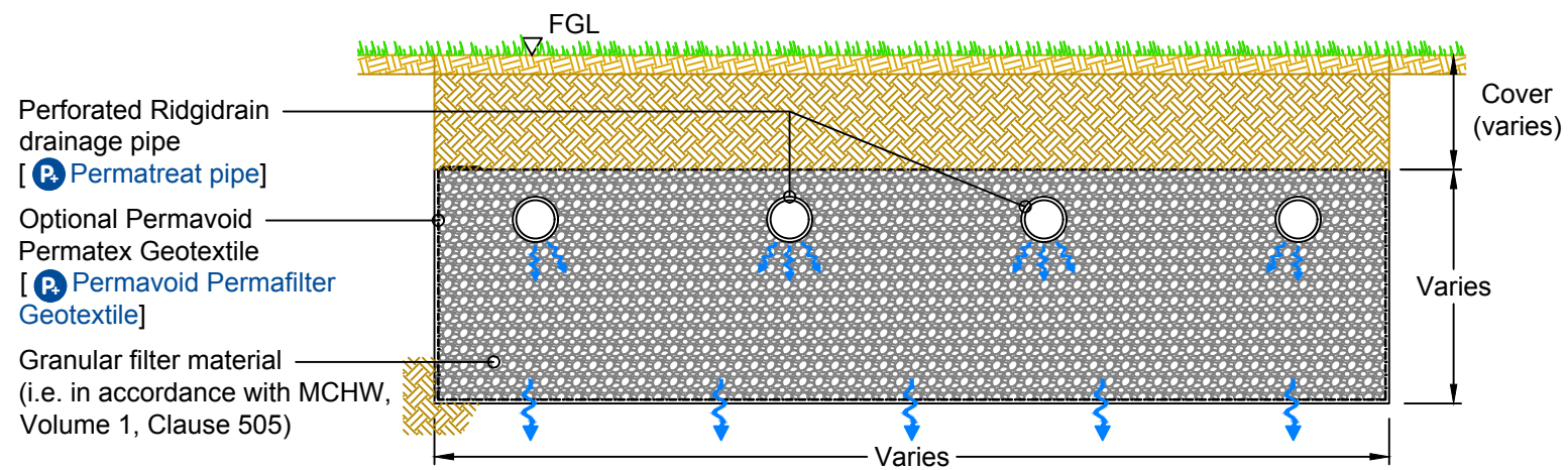
TYPICAL SECTION
